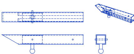
MAST STEP
