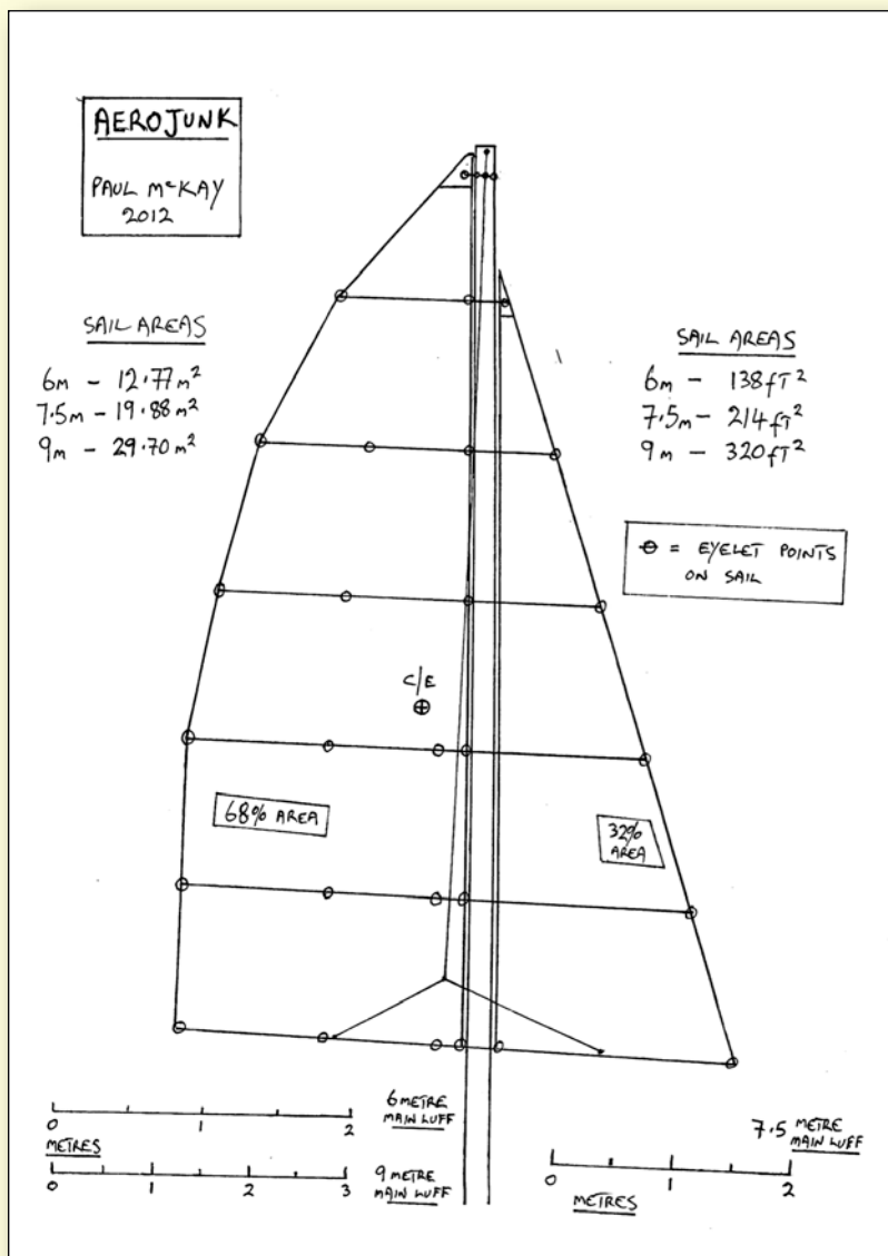
The Aerojunk planform
